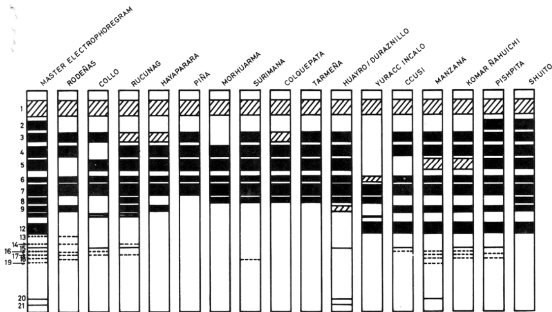
Fig. 2. Electrophoregrams of S. × chaucha morphotypes. Faint or diffuse bands are indicated by dotted lines and cross-hatching.
